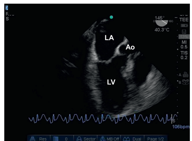
Figure 6 – Midesophageal three-chamber view. See Figure 1 and 2 legends for expansion of abbreviations.
